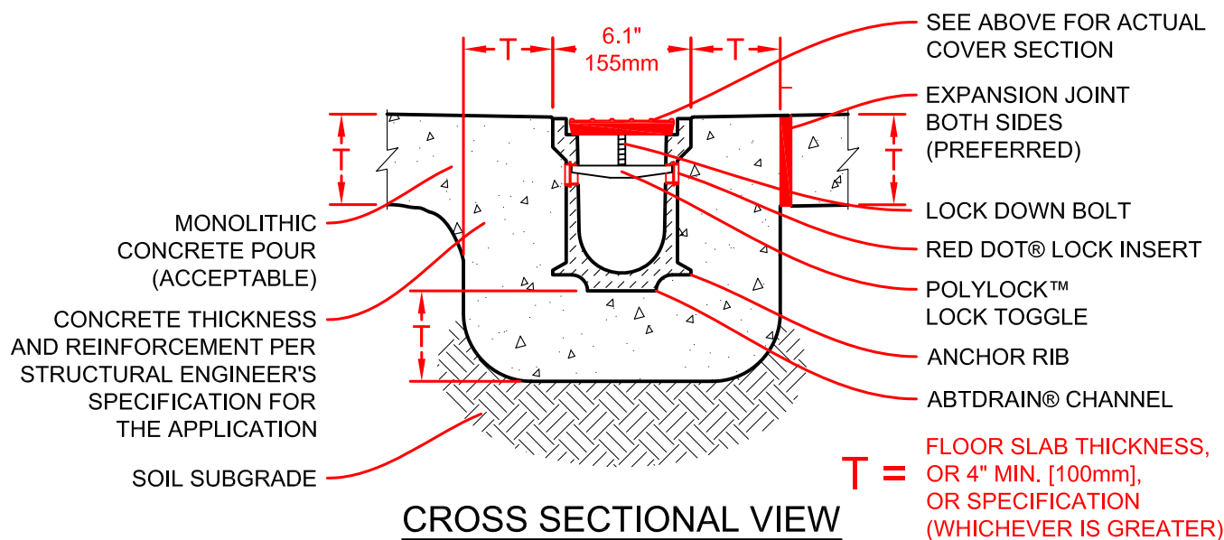
SECTION
